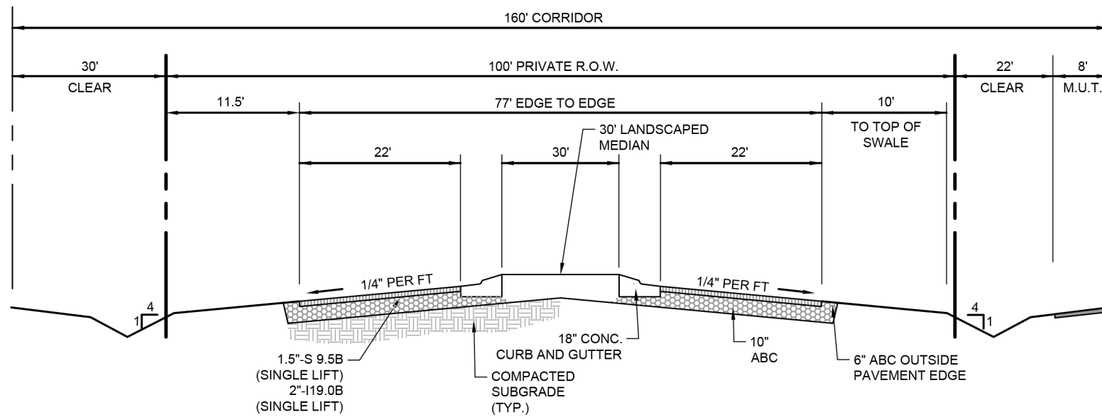
TYPICAL 100' PRIVATE R.O.W. SECTION (DIVIDED PARKWAY) NOT TO SCALE
