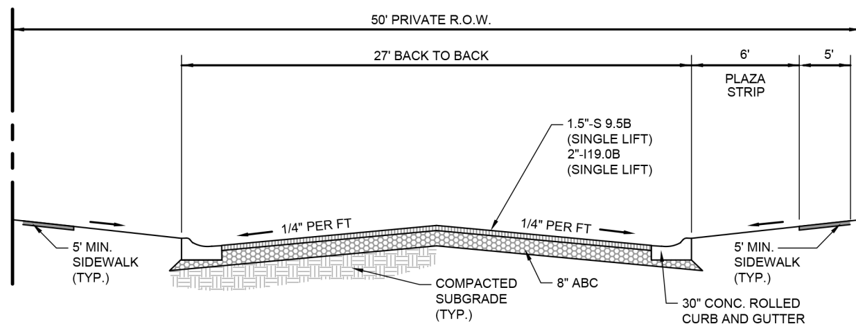
TYPICAL 50' PRIVATE R.O.W. SECTION NOT TO SCALE
