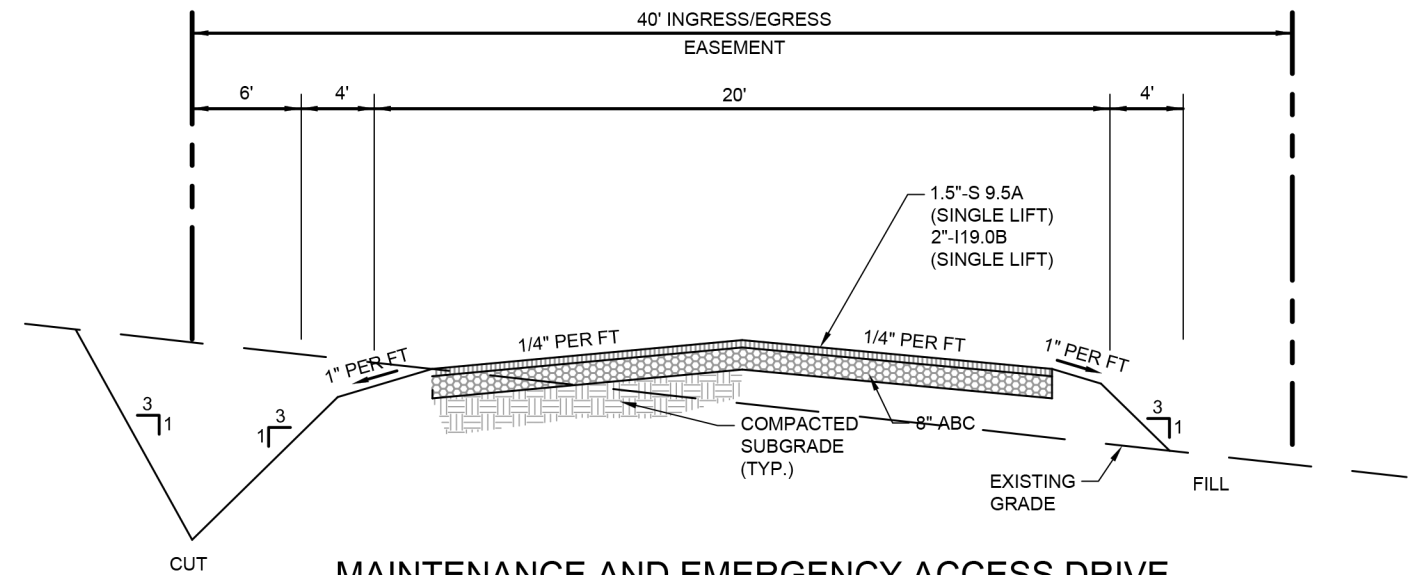
MAINTENANCE AND EMERGENCY ACCESS DRIVE NOT TO SCALE
