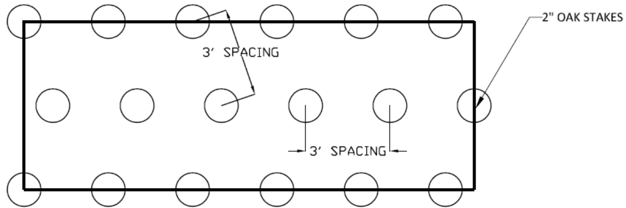
MATTING STAKES PLAN VIEW
