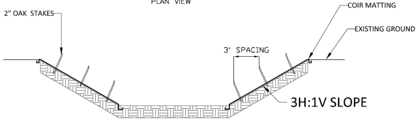
SECTION VIEW
