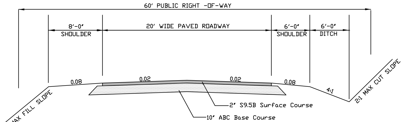
Typical 20' Edge to Edge Section (not to scale)
