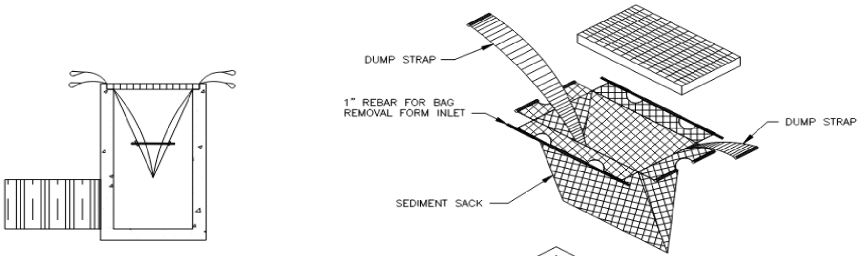
INSTALLATION DETAIL
