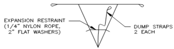
BAG DETAIL
