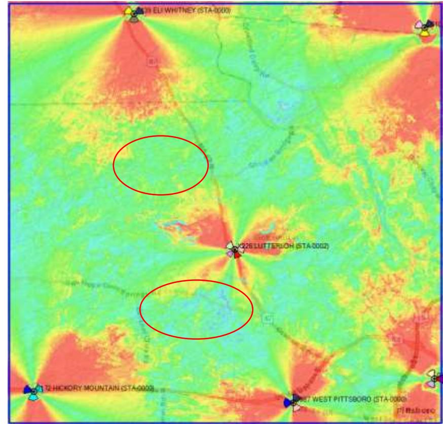
C/L AFTER (199')
