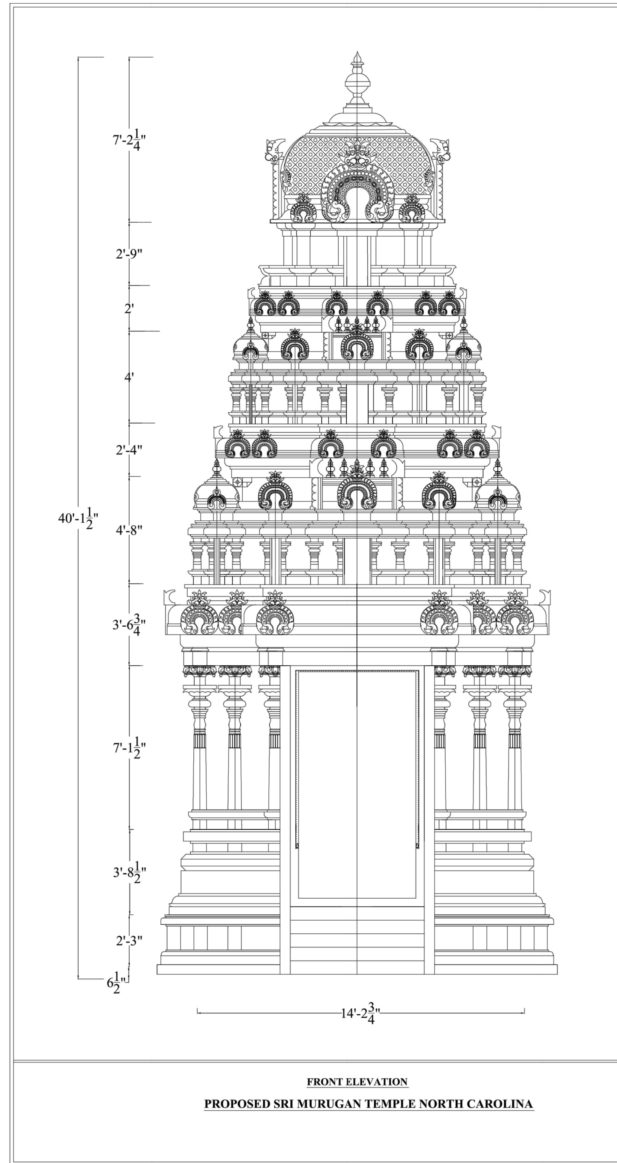
1 TEMPLE ENTRANCEWAY ELEVATION (BY OTHERS) D-102 NTS
