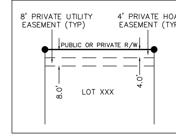
PRIVATE EASEMENT DETAIL
